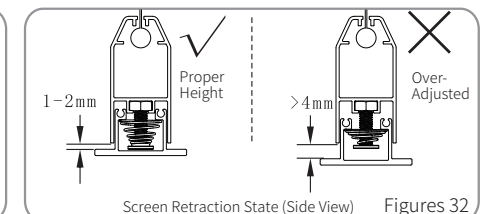
Screen Retraction State (Side View) Figures 32
